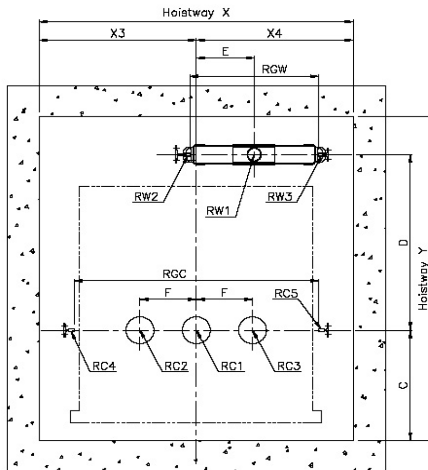
Hoistway Plan
