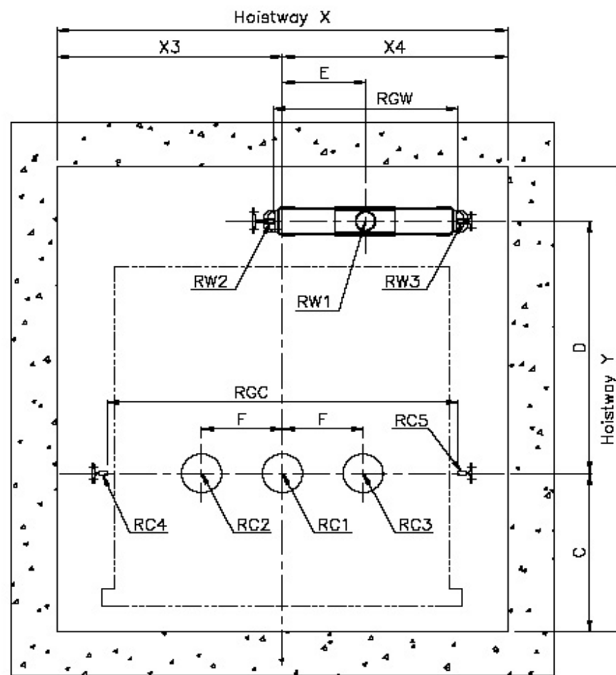
Hoistway Plan
